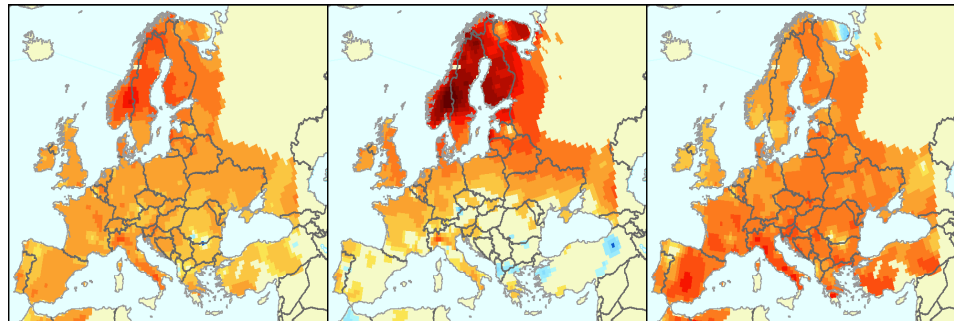
Observed temperature change over Europe during the period 1976–2006
