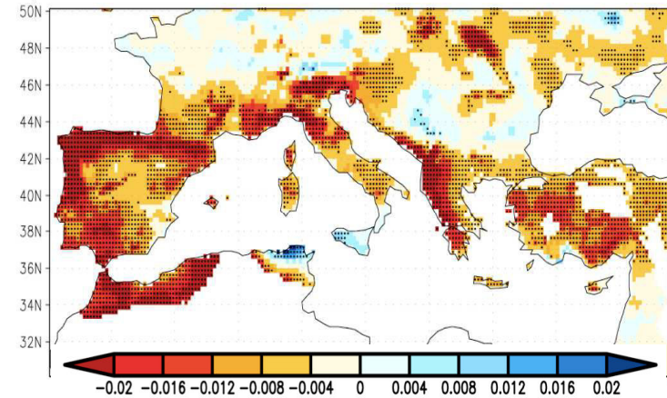
b) E-OBS ANNUAL MEAN PRECIPITATION. LINEAR TREND, 1960–2008
